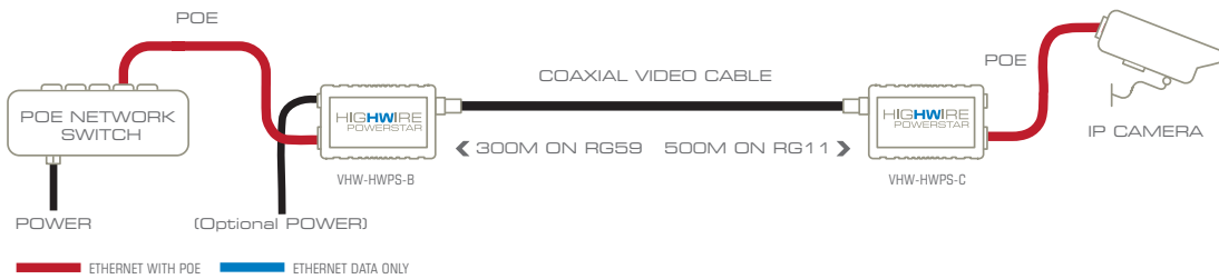
Diagram 1. HIGHWIRE Powerstar delivers Ethernet and POE over legacy coax, for maximum reliability with minimal wiring.
